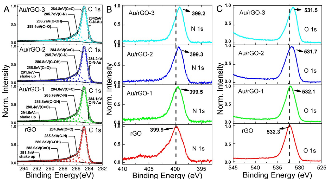
Figure 2. (A–C) XPS spectra of the C 1s region, N 1s region, O 1s region of rGO, Au/rGO-1, Au/rGO-2, and Au/rGO-3, respectively. Synthesis conditions: Au/rGO-1 (0.5 mM HAuCl 4 ), Au/rGO-2 (1 mM HAuCl 4 ), Au/rGO-3 (2 mM HAuCl 4 ) in 0.17 mg/mL rGO solution; room temperature; 1 h.
